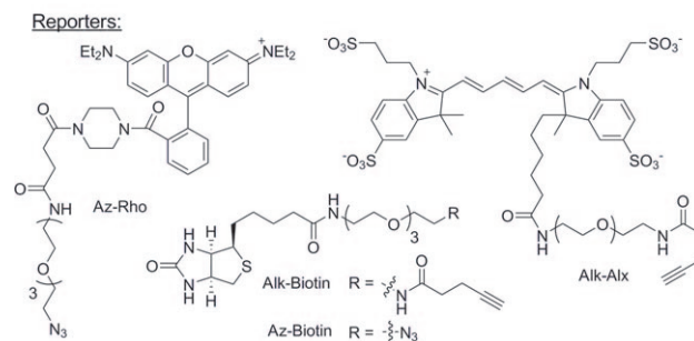
Scheme 1. Methionine surrogates (blue) and unnatural metabolite PTM probes (orange) form bio-orthogonal pairs for compatible double metabolic incorporation. Those forming pairs are boxed in the same group. Azide- and alkyne-containing fluorophore and biotin reporters are also shown (bottom).
